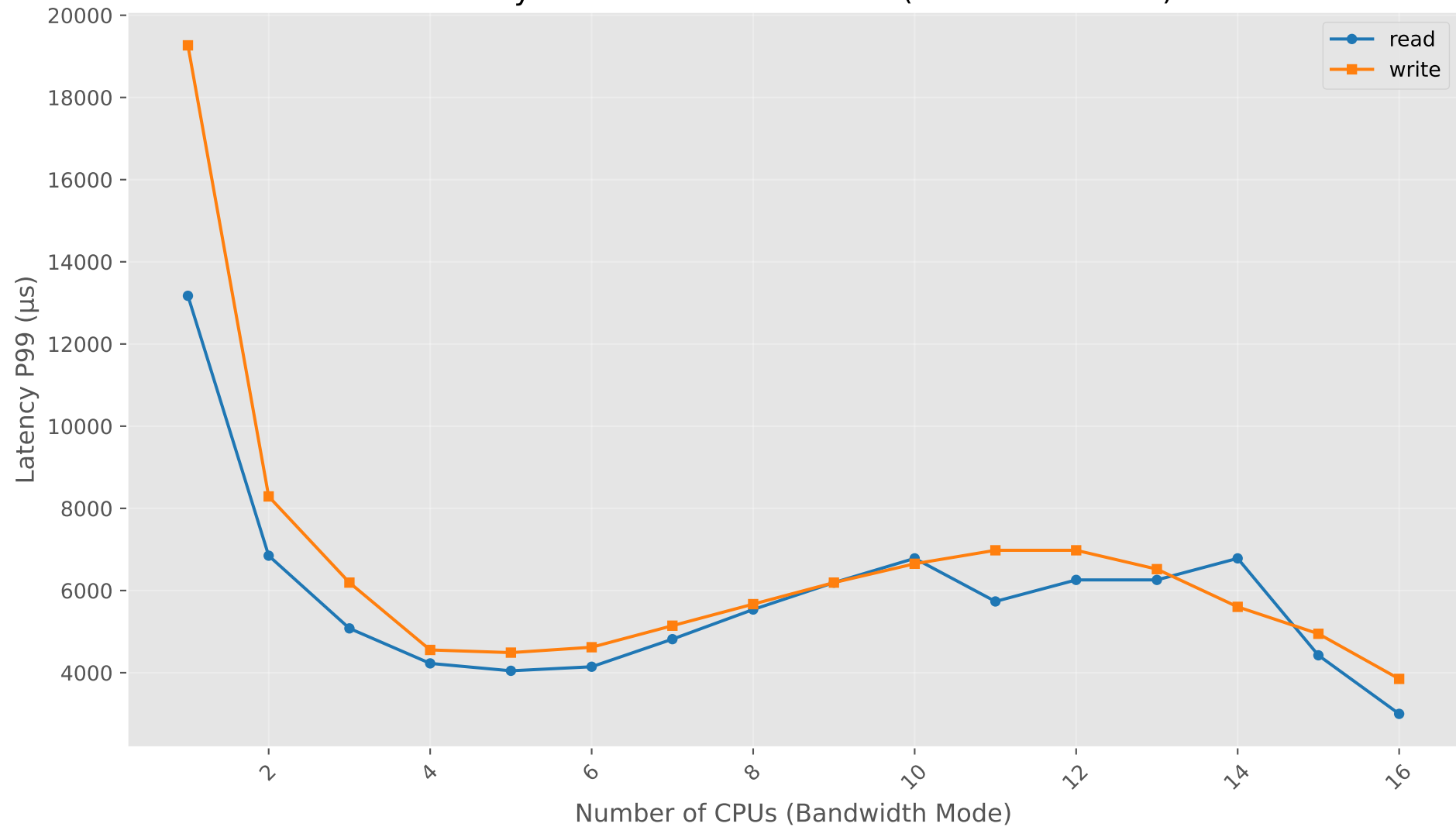
Latency P99 vs Number of CPUs (Bandwidth Mode)
